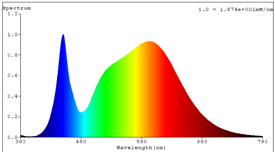
Spectral Distribution
